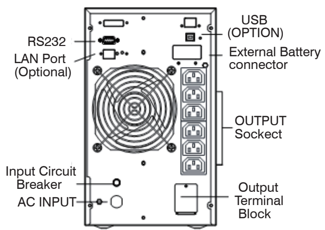
CNH110-3KS_HV Rear Panel
