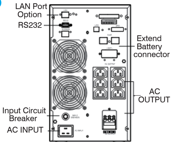
CNH110-3K_HV Rear Panel
